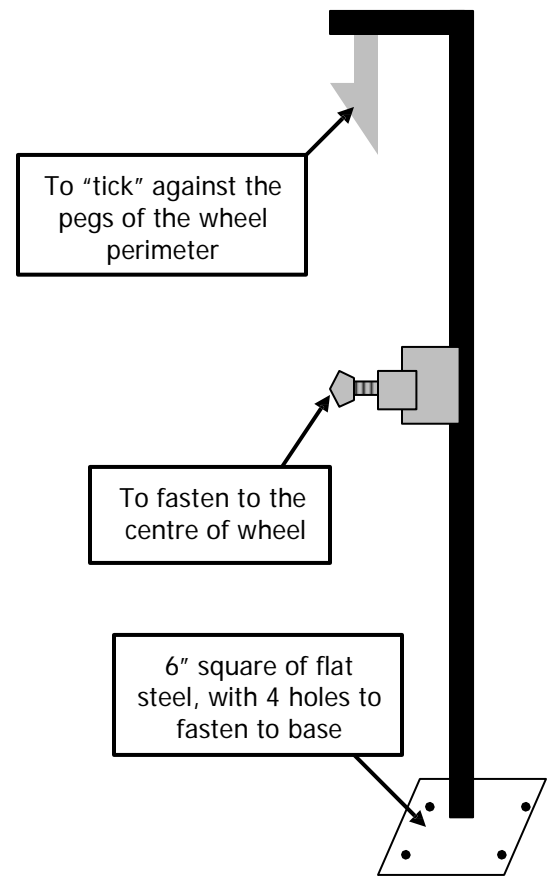
Wheel Mount
